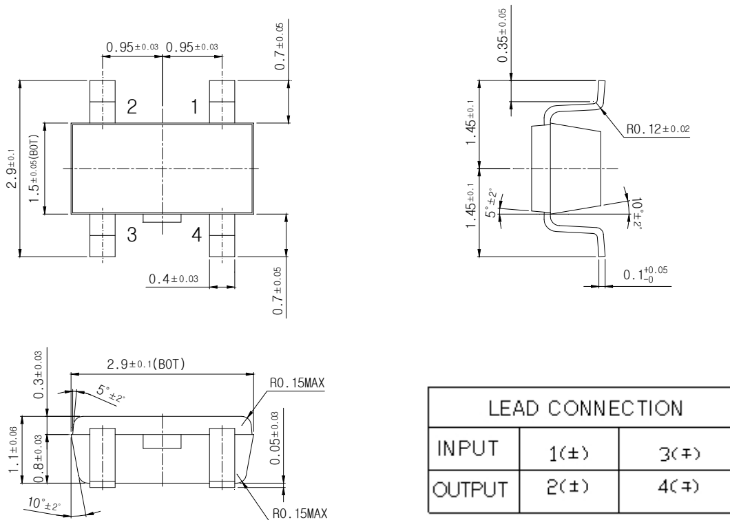
[Package Dimensions]
